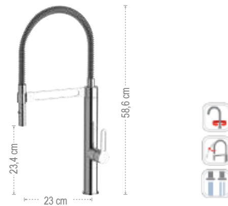
SR513 Miscelatore lavello con flessibile nero rivestito con molla "fine design". Sink mixer with black flexible hose coated with "fine design" spring.
