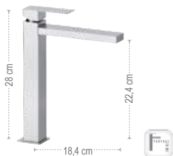
Miscelatore monocomando lavabo alto LXL. Single-lever LXL high washbasin mixer.
