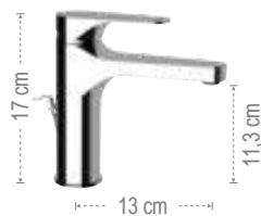
Miscelatore monocomando lavabo alto L. L high single lever basin mixer.
