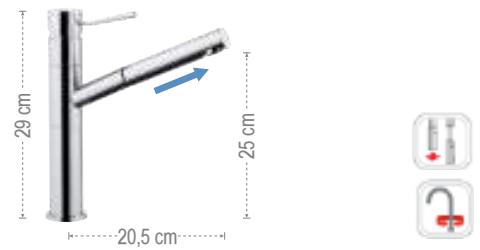
N47 Miscelatore monocomando per lavello, con bocca estraibile e girevole. Single-lever one-hole sink mixer, with pull-out spray jet shower with swivel spout.
