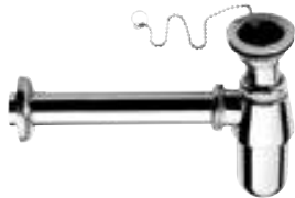
973Z Sifone a bottiglia in zama con pileta, per lavabo, 1" 1/4". Bottle trap in zamac with waste, for wash-basin, 1" 1/4".
