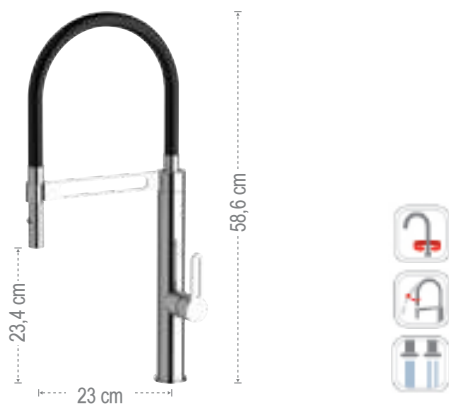
SR511 Miscelatore lavello con flessibile rivestito in tubo gomma soft-touch nero opaco. Sink mixer with flexible hose coated in soft-touch matt black rubber pipe.
