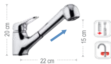
K47M Miscelatore monocomando monoacqua per lavello, con doccia estraibile a getto variabile. Single-lever single water one-hole sink mixer, with pull-out spray jet shower two functions.
