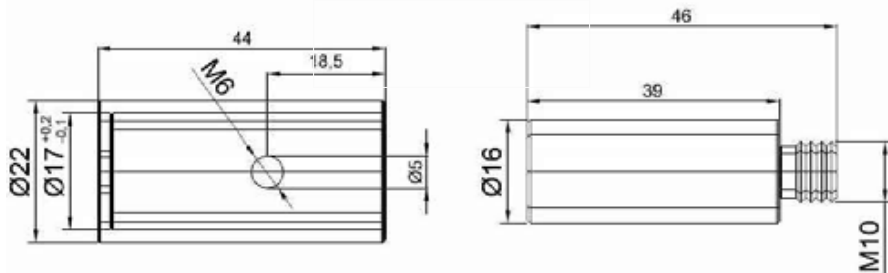
MOUNTING BRACKET
